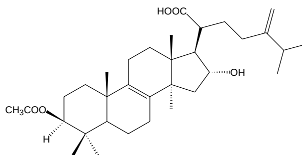
Fig. 1. Structure of pachymic acid.
